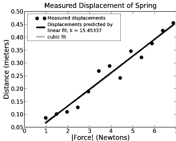
Figure 18.9 A model up to the elastic limit
